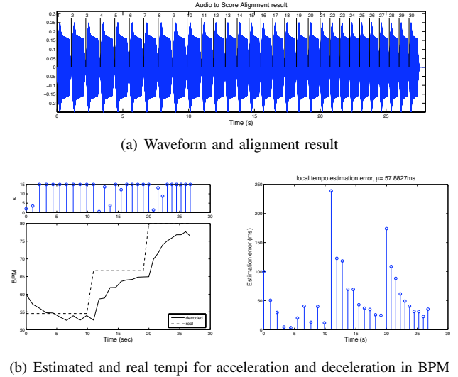
Fig. 10. Evaluation of tempo decoding using synthesized score and discretely controlled tempo.
