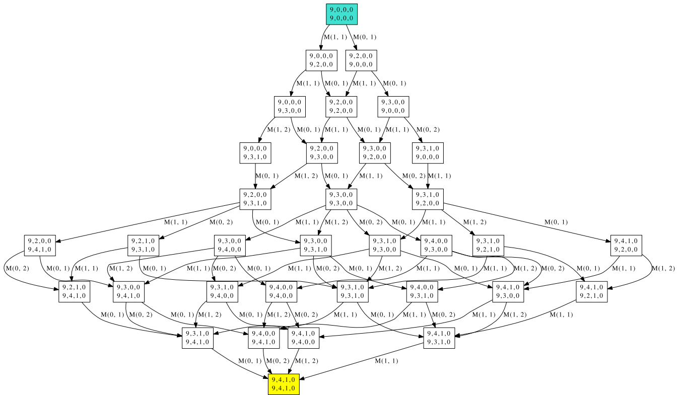
Fig. 10. The transition system of a quorum sensing process for two rows of cells on a square grid.
