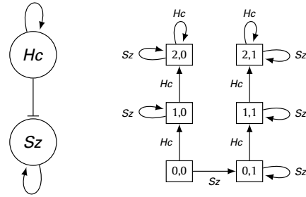
Fig. 1. Left: the formal definition of a simple regulatory network for one cell of Anabaena . Middle: its graphical abstract representation. Right: the corresponding state space where each node is a state labeled by x_{Hc} , x_{Sz} and each edge corresponds to the change of one variable as indicated in its label.
