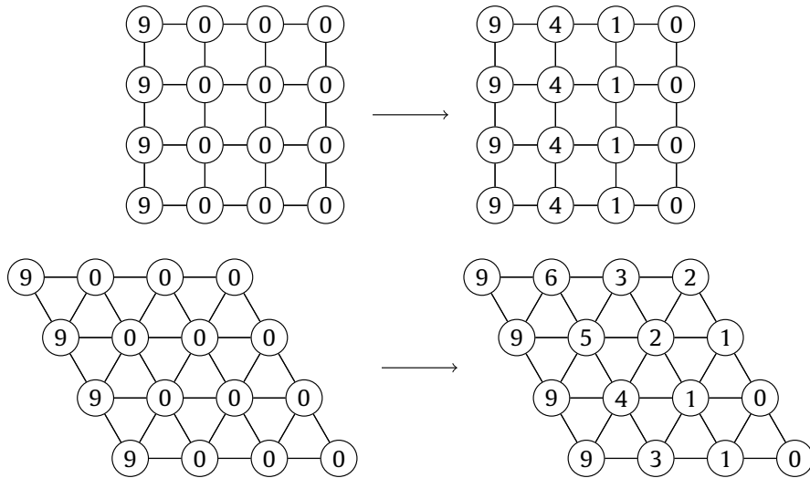
Fig. 9. Each row shows the initial and final state of a quorum sensing process. Only the declaration of the underlying spatial representation changes between the two rows: exactly the same variables, update functions and implementations have been used.
