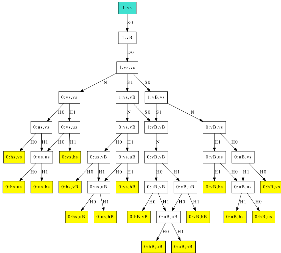
Fig. 7. The transition system generated from the initial state corresponding to a single small vegetative cell and x_{Nitro} \stackrel{df}{=} 1 , with both parameters Nbr_m and Nbr_N set to 2. Each state is depicted as a rectangle whose label gives first x_{Nitro} then, for each module, the value of each local variable Hc and Sz encoded by the initial character of the corresponding symbol. For example, 0:hB,vs stands for an IRN state with \lambda \stackrel{df}{=} \{Nitro = 0\} and C \stackrel{df}{=} \{Hc = heterocyst, Sz = big\} , \{Hc = vegetative, Sz = small\} (two vertexes linked by comma operator). There is an edge between two nodes iff a corresponding transition exists. Edge labels are either H_i , S_i or N , corresponding respectively to an evolution of Hc , Sz in module i , or Nitro globally. Leaf nodes in this directed acyclic graph (there is no periodic behavior) are stable states.
