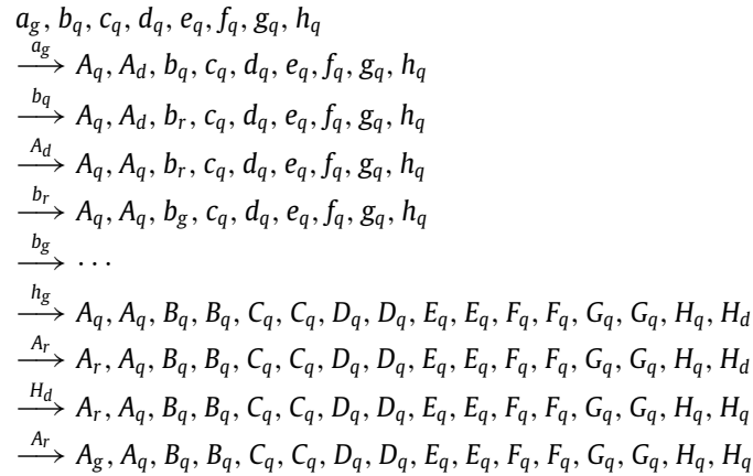
Fig. 6. A complete evolution of an IRN encoding a DOL system with rules such that each letter is replaced by two copies in upper case. The value of the flag is given by the subscript, the left-most cell is the one starting the word and the ring is left-right oriented.
