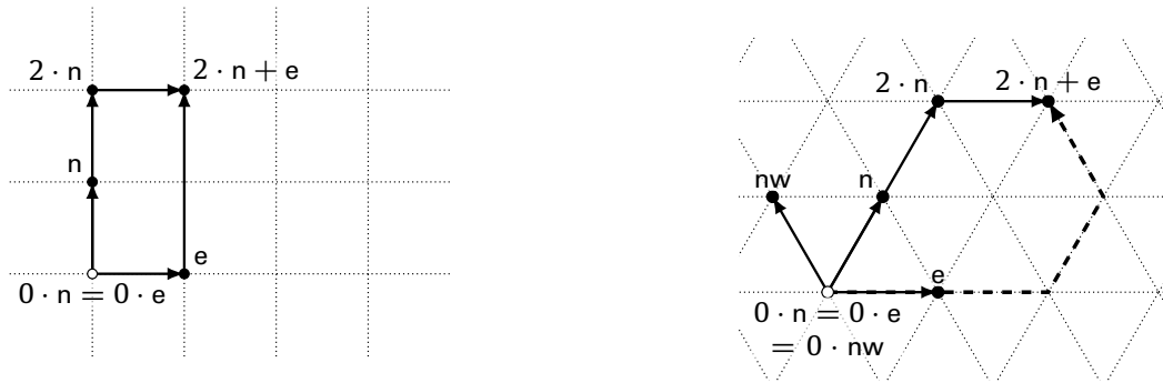
Fig. 8. Left: a GBF defining a square grid, with two generators e and n . Right: a GBF defining a hexagonal grid with three generators e , n and nw , and a constraint n - nw = e .
