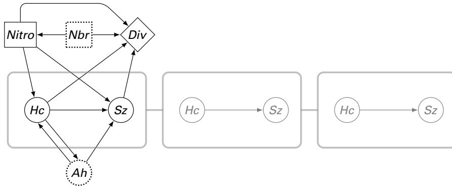
Fig. 5. In black: graphical representation of the IRN specification of Anabæna ; in the upper part, global variable Nitro , global measure Nbr and graph update Div ; in the middle part, local variables Hc and Sz ; in the lower part, local measure Ah . In gray, a view of a linear graph C with three vertexes with the corresponding local variables.
