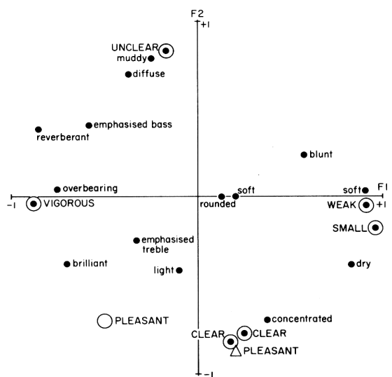
FIG. 9. Representation of Factor Plane F1-F2. The bipolar rating scales taken for the interpretation of factors indicated ●. The quality evaluations of the two groups are indicated △, ○.
