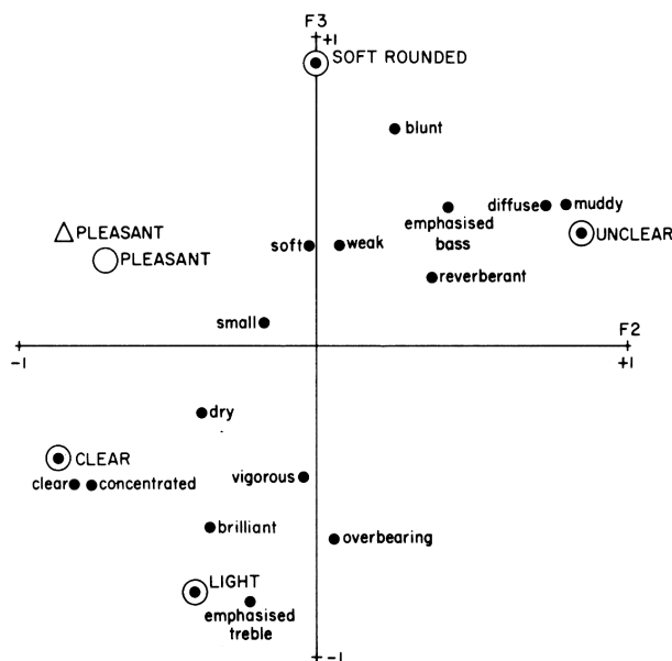
FIG. 10. Representation of Factor Plane F2-F3. The bipolar rating scales taken for the interpretation of factors are indicated ●. The quality evaluations of the two groups are indicated △, ○.
