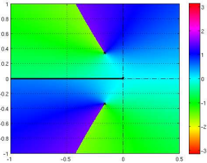
Fig. 3. Phase of \Gamma(s) , as defined by (46), ( \beta = 2 ).
